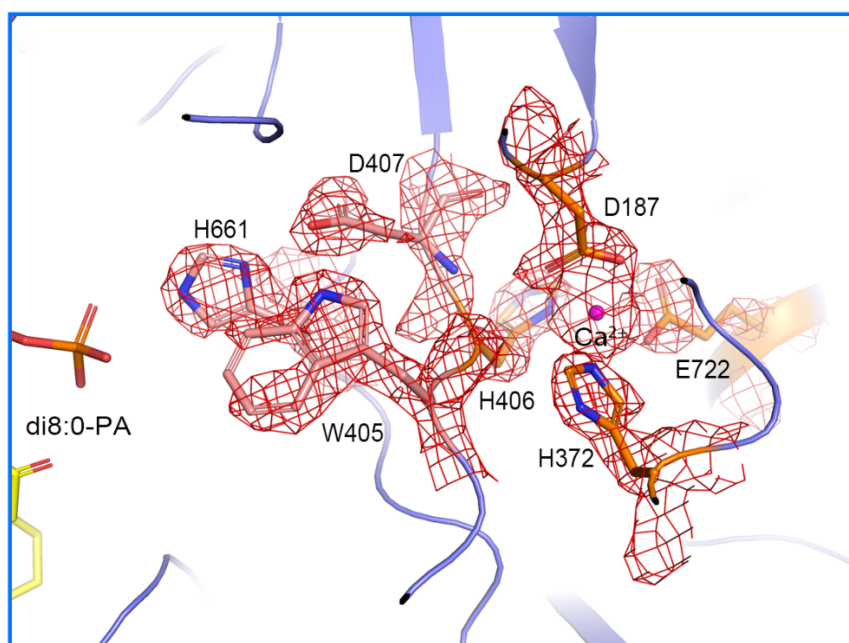
Figure S10. Electron density of Ca 2+ binding site and coordinating residues near the active site. (Contoured at 1.5σ)
