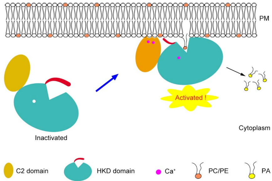
Figure S13. A simplified functional model of C2-PLD. In the inactive state, the lid of the substrate-binding pocket of C2-PLD adopts a closed conformation to seal the pocket; when C2-PLD attaches to the membrane and the Ca 2+ binds, the lid opens up to allow the membrane lipids entering into the pocket.
