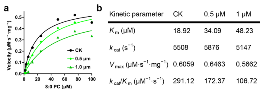
Figure S1. In vitro kinetic assay to show the competitive inhibition of Bazedoxifene toward PLD \alpha 1 (di8:0-PC as substrate). a Michaelis-Menten kinetics of PLD \alpha 1 in the presence of different concentrations of Bazedoxifene, 0 \mu\text{M} (CK, black), 0.5 \mu\text{M} (green), and 1 \mu\text{M} (olive). b The kinetic parameters were calculated and shown in the table. The experiments were repeated three times with similar results.
