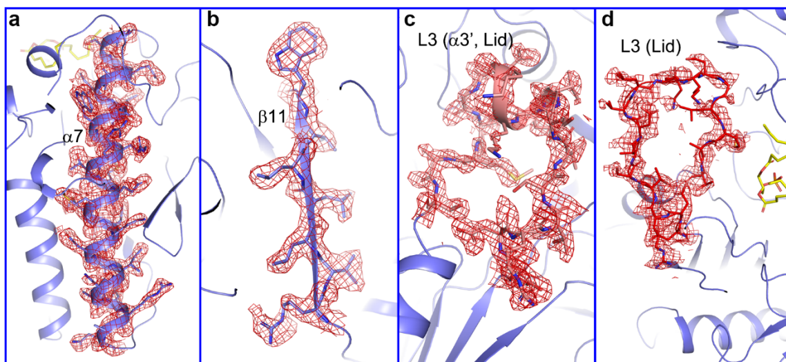
Figure S2. Representative electron density of PLD \alpha 1 contoured at 1.0\sigma . a-c
