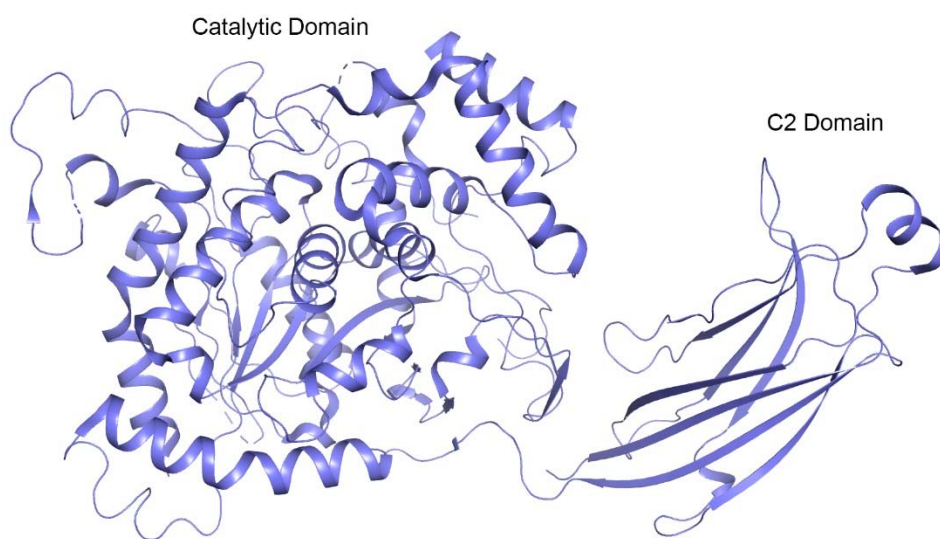
Figure S3. Structure of human cPLA2 (PDB ID: 1CJY)
