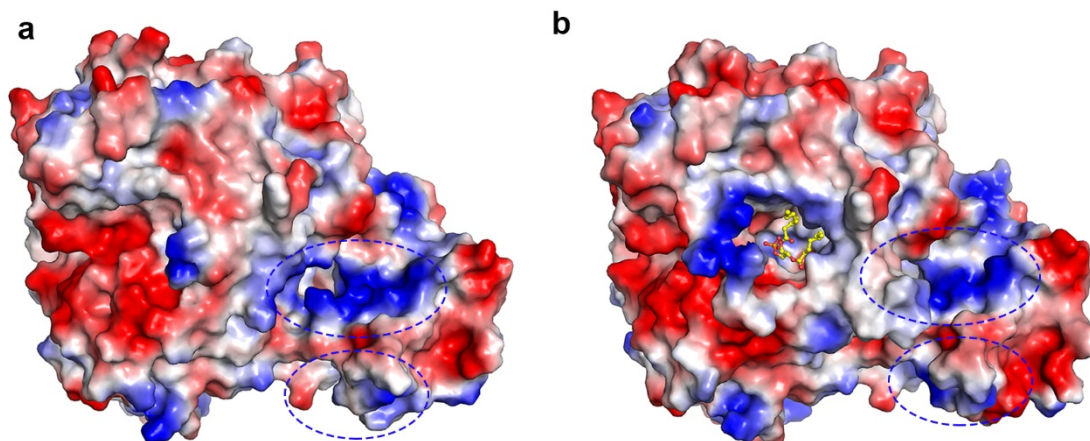
Figure S5. Electron static surface model show the close and open conformation of the substrate-binding pocket. a Close conformation of substrate-binding pocket in the apo-PLD \alpha 1 structure. b Open conformation of substrate-binding pocket in the PLD \alpha 1-PA complex structure. PA is shown with a stick model. The positive-charged patches are circled with dotted line. Red color and blue color indicate the negative and positive charges.
