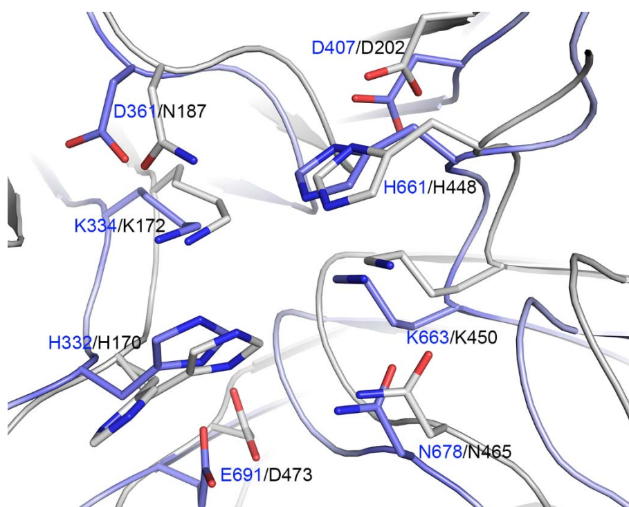
Figure S9. Comparison of the active site residues in PLD \alpha 1 and PLD PMF structures.
