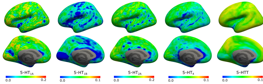
Supplementary Figure 1: Standard deviation maps of mean normalized BP ND bootstrap samples. Maps are displayed on the lateral (top) and medial (bottom) views of the fsaverage surface (left hemisphere, inflated)
