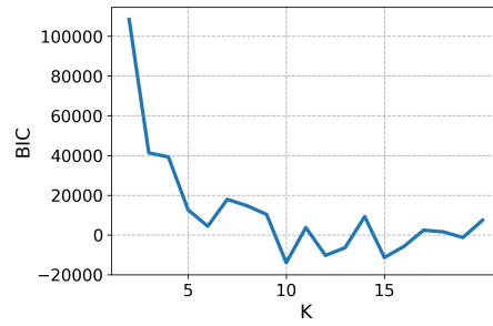
Supplementary Figure 2: Bayesian information criterion (BIC) associated with the parcellations obtained with K clusters. A minimum indicating an optimal model is found at K = 10 .
