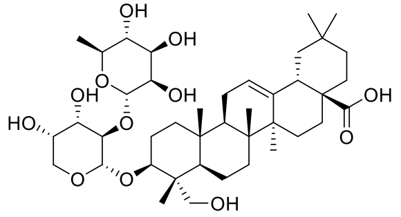
Sapindoside A
