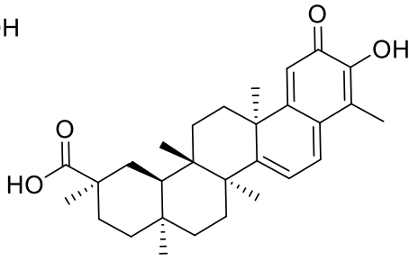
Celastrol
