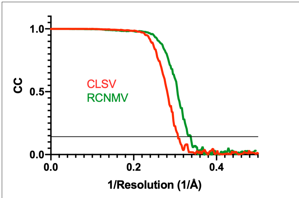
Figure S1: Gold standard Fourier shell correlation (FSC) curves for the two viral cryo-EM models. The black line shows the standard correlation coefficient cutoff of 0.143
