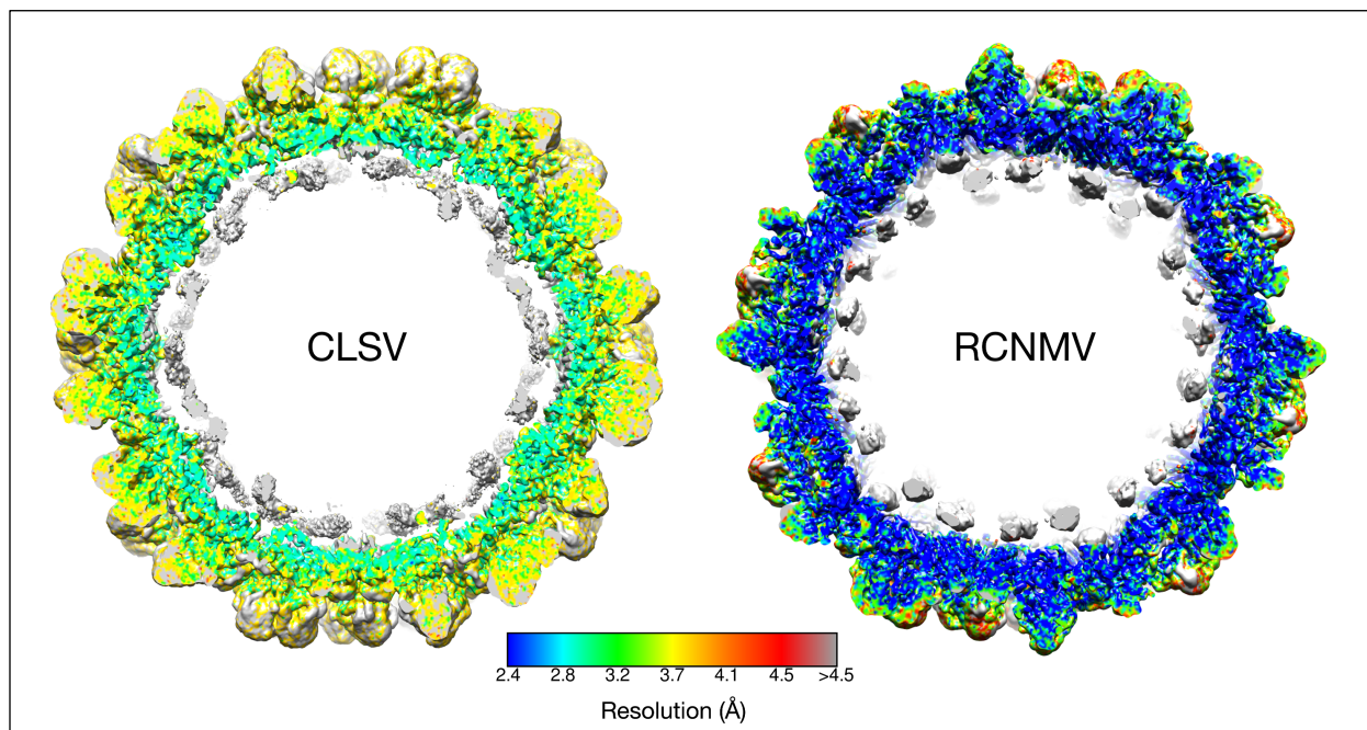
Figure S2: Local resolution maps of the two reconstructions. Shown here are the cutaway midsections of the two reconstructions analyzed with ResMap (1). The color key of each resolution range is shown at the bottom.
