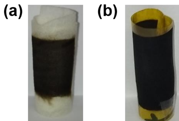
Figure S2. The good resistance of twisting demonstrated by the graphene coated substrates: (a) non-woven fabric and (b) polyimide.
