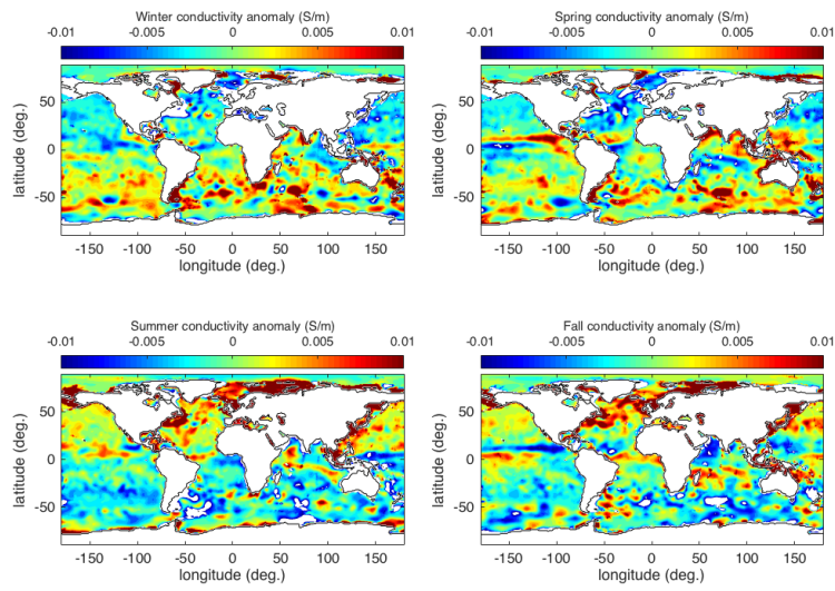
Fig S1: Depth-averaged conductivity anomaly (relative to annual mean) for each of the four seasons. The full range in the data are, respectively, -0.660 — 0.556 (S/m), -0.471 — 0.317 (S/m), -0.511 — 0.721 (S/m), -0.502 — 0.594 (S/m).
