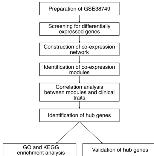
Figure S1. Flow chart of data preparation, processing, analysis and validation as performed in the current study. GO, Gene Ontology; KEGG, Kyoto Encyclopedia of Genes and Genomes.
