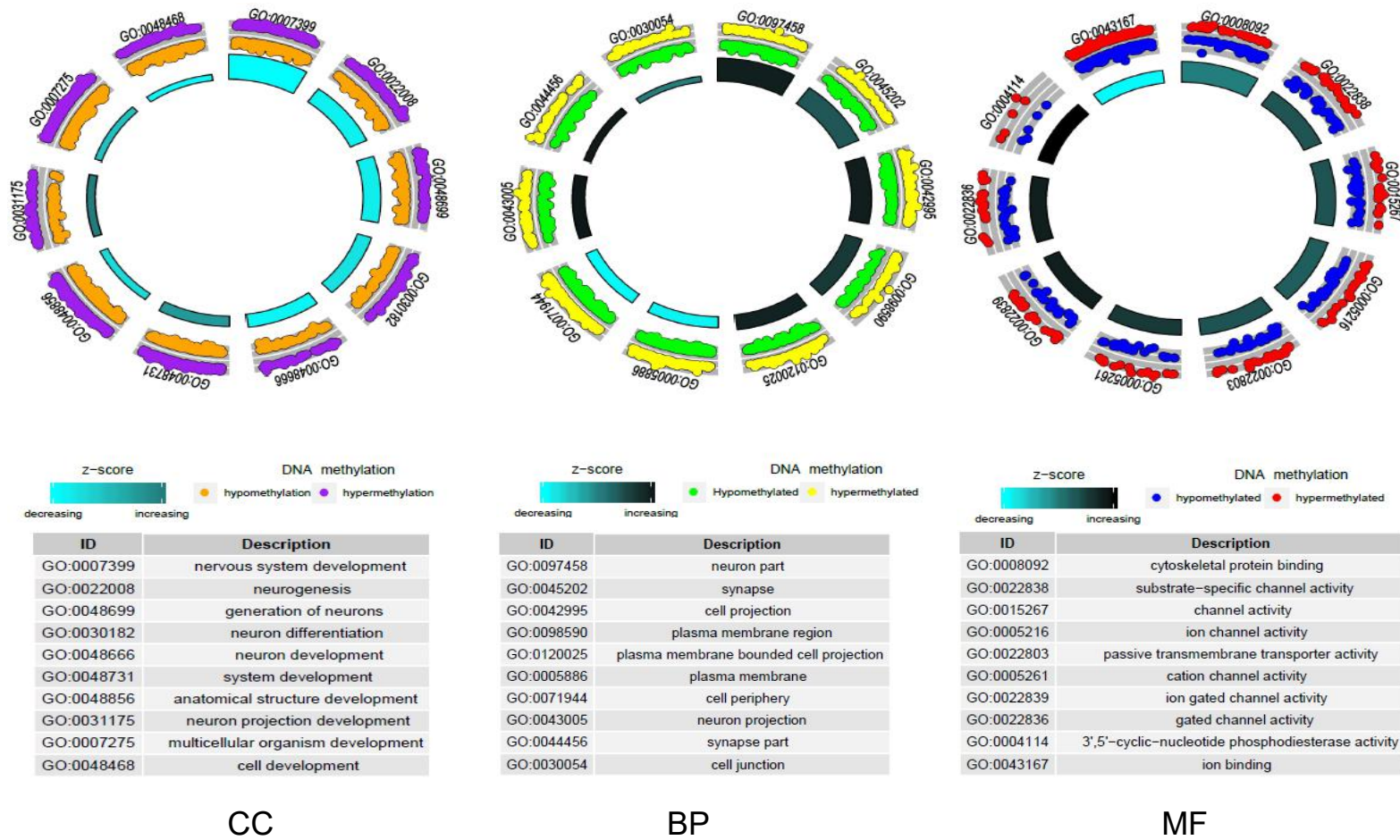
Supplementary Figure 4. GO terms enrichment analysis of DMGs. The z-score indicates the Difference value between counts of hypermethylated and hypomethylated genes in each GO term.
