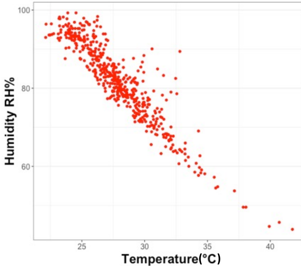
Figure S1. Relationship between observed temperature ( ^{\circ}\text{C} ) and relative humidity (%). Red dots represent individual observations per hour recorded.
