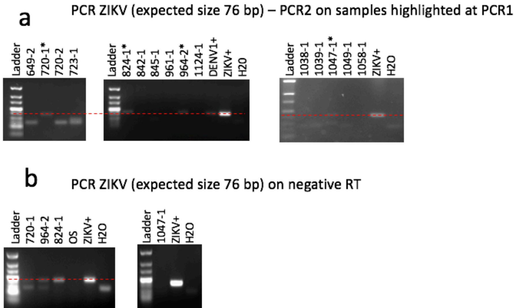
Figure S6. Visualization of the second PCR products of ZIKV on agarose gels. Expected size of positive fragments: 76 bp. ZIKV+: positive control.
