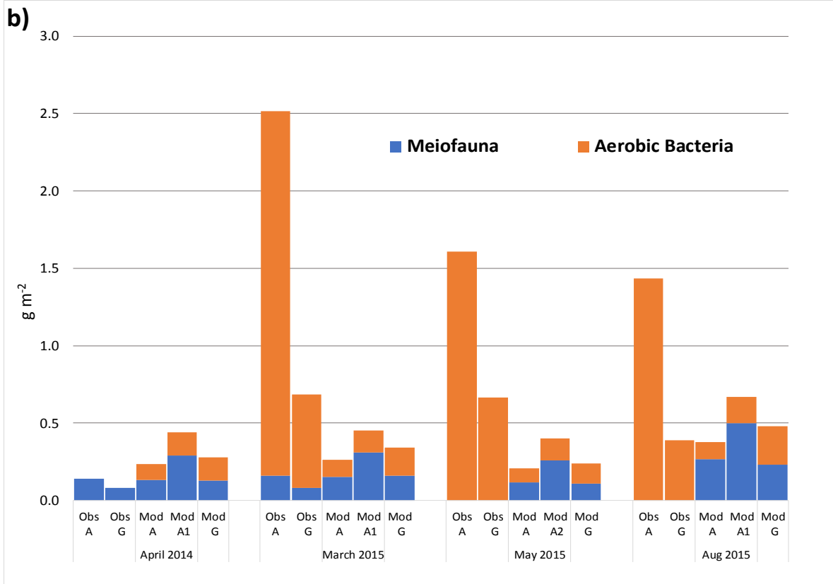
Figure b: Meiofaunal and aerobic bacteria biomass ( \text{g C m}^{-2} ) model-data comparison at sites A and G. Observations replicate means (5 samples).
