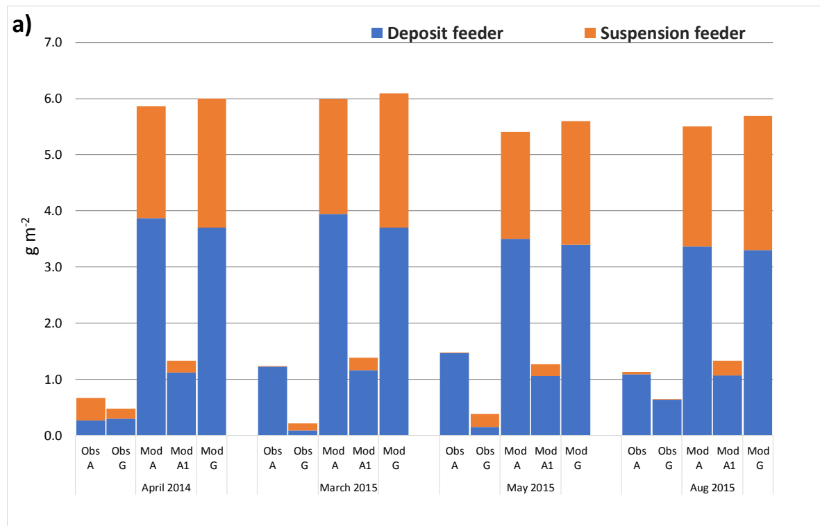
Figure a: Benthic macrofauna model-data comparison at sites A and G. Observations replicate means (5 samples).
