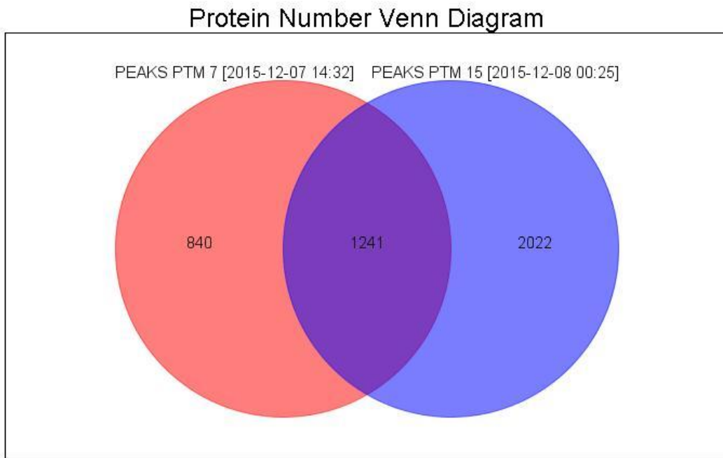
Fig B. Venn diagram of protein score distribution and protein numbers in tumor and adjacent normal tissues for stage 2.
