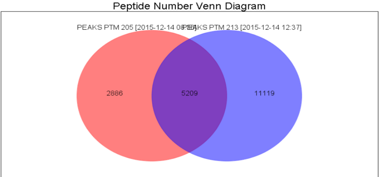
Fig C. Venn diagram of peptide score distribution and protein numbers in tumor and adjacent normal tissues for stage 3
