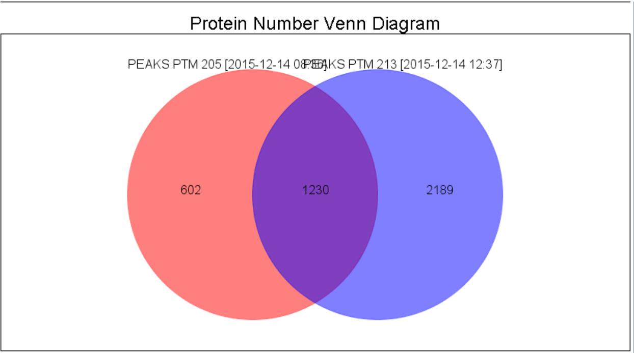
Fig D. Venn diagram of protein score distribution and protein numbers in tumor and adjacent normal tissues for stage 3
