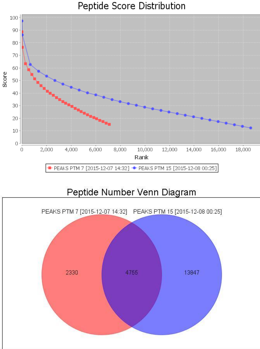
Fig A. Venn diagram of peptide score distribution and numbers of tumor and adjacent normal tissues for stage 2. (Blue colour is tumor and red colour is normal)
