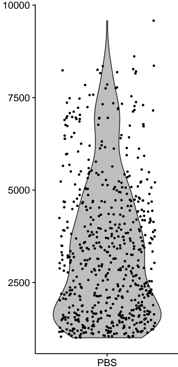
Identity
