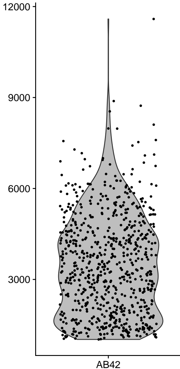
Identity
