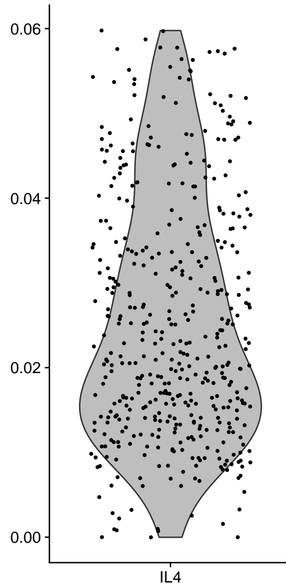
percent.mito
