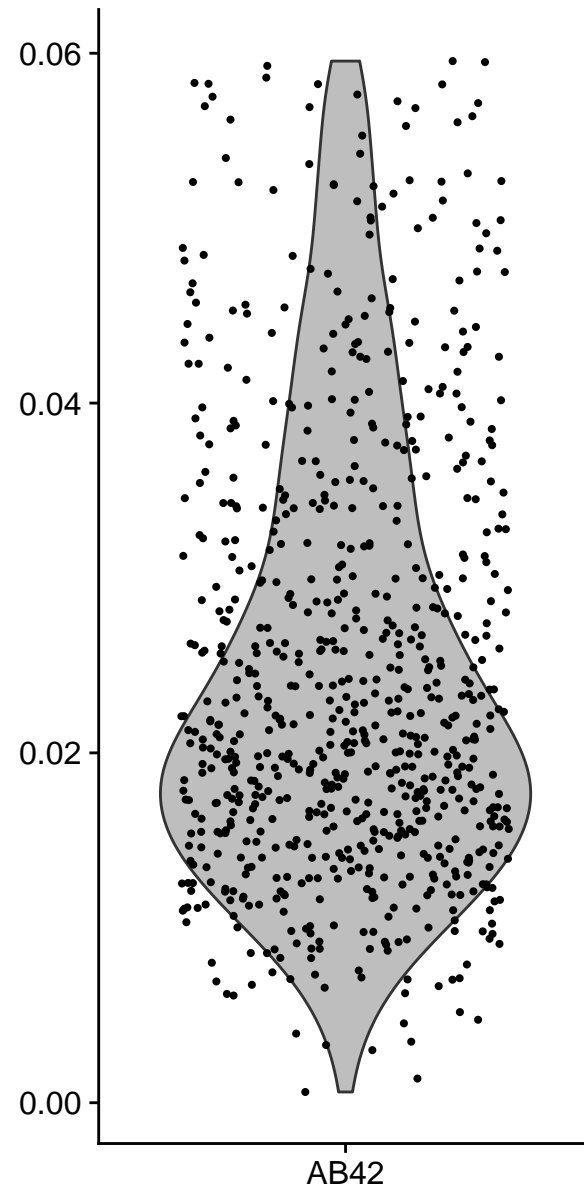
Identity
