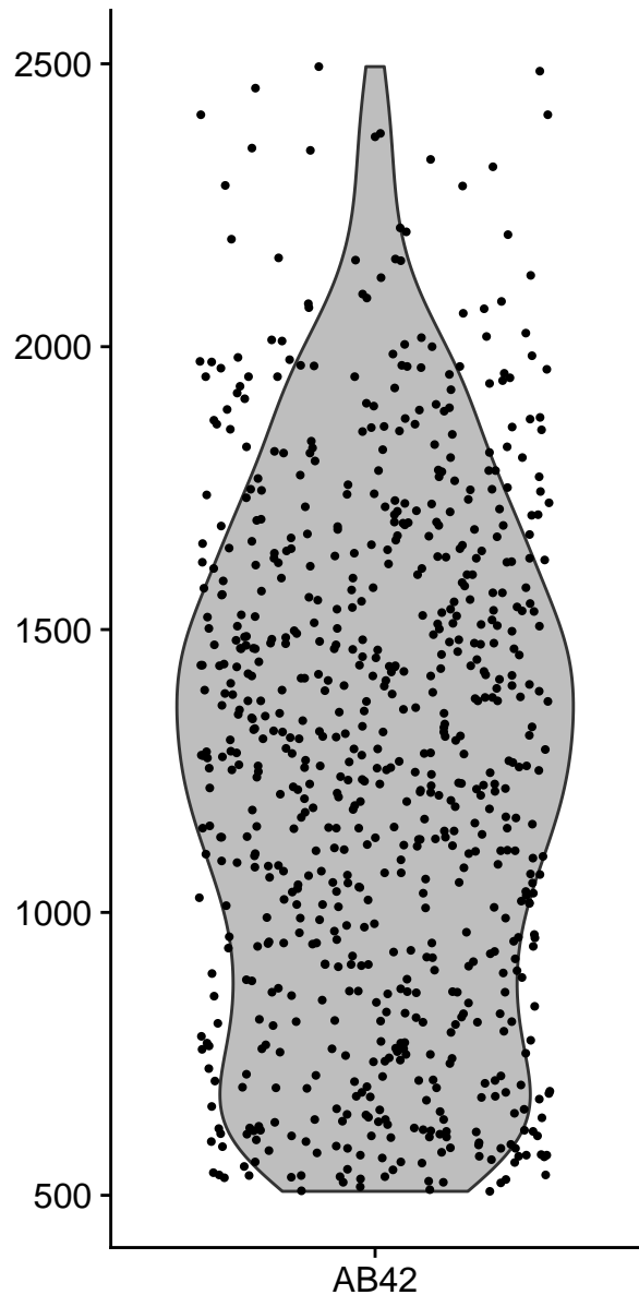
Identity
