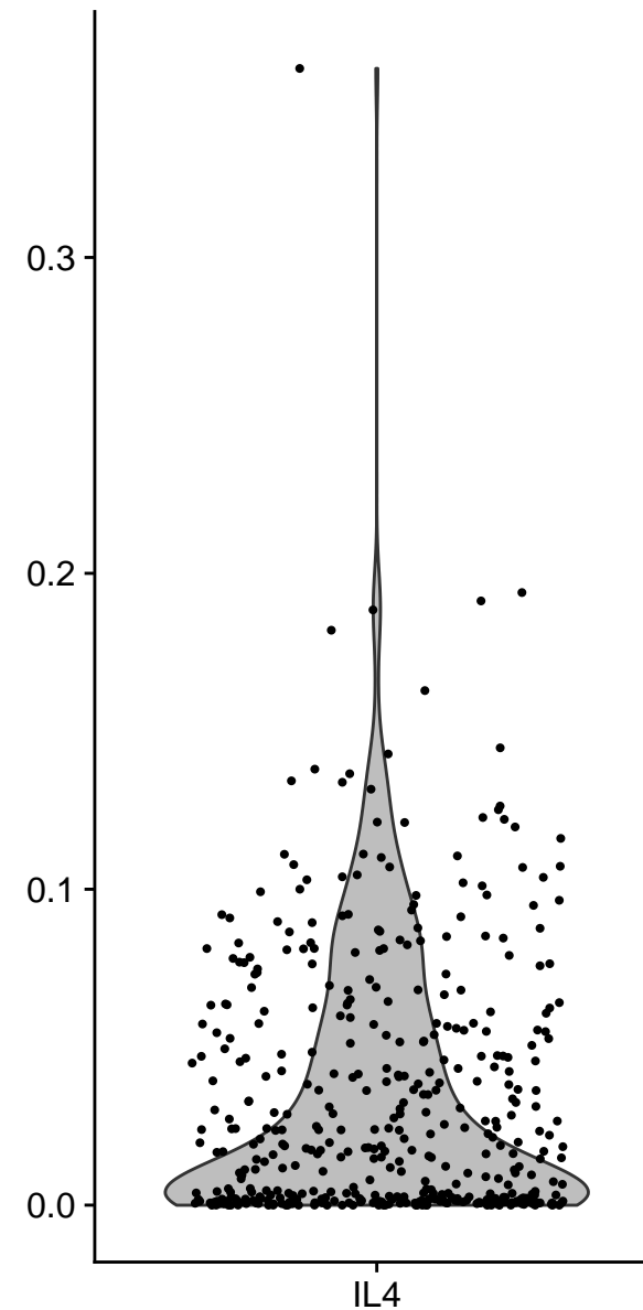
percent.gfp
