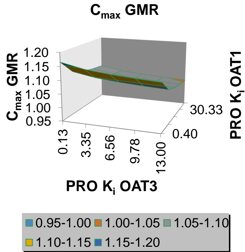
Figure S4. Sensitivity analysis on PRO OAT1 and 3 K i value and its effects on TFV plasma pharmacokinetic parameters TFV AUC 0-∞ geometric mean ratio (GMR), C max GMR, and renal clearance (Cl r ).
