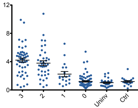
SEMG1
