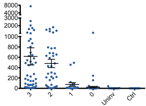
TRNP1
