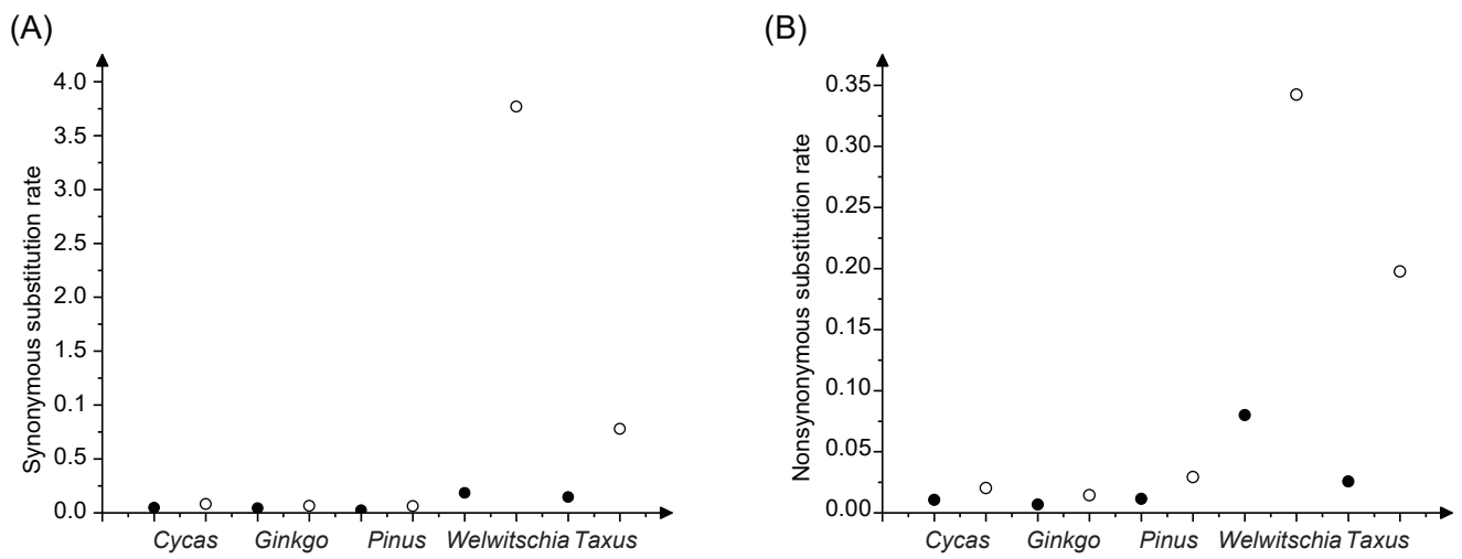
Additional file 14: Figure S8. Synonymous (A) and nonsynonymous (B) sequence divergence in the conserved region of mitochondrial protein-coding genes in gymnosperms. Dots indicate mitochondrial protein-coding genes that have not transferred to the nucleus in all five gymnosperm species. Circles indicate the transferred genes in Taxus and Welwitschia and their homologous genes in Cycas , Ginkgo and Pinaceae.
