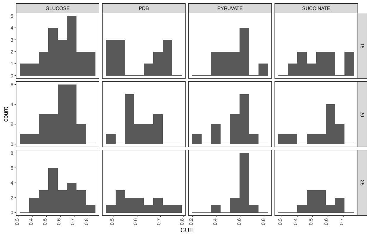
Figure S2: Frequency histograms of CUE of isolates grown on the four substrates at three temperatures. Each count is the average of all replicates for a given isolate under that assay condition.
