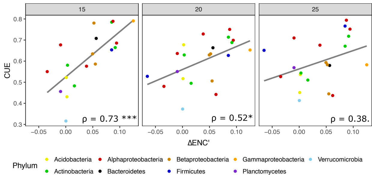
Figure S7: Correlations between CUE and codon bias (as per (41)) for bacterial isolates grown on glucose. Spearman correlation coefficients (not corrected for phylogenetic correlation) are included, along with the p-value (***) P < 0.001 ; * P < 0.05 ; . P < 0.1
