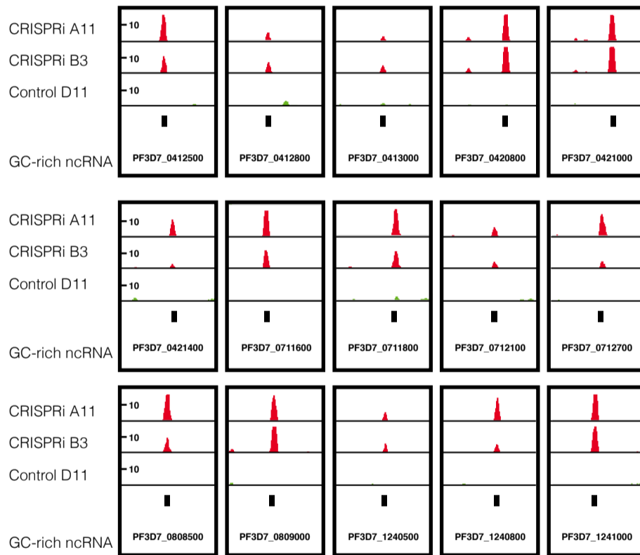
dCas9 ChIP at GC-rich genes at 24hpi
