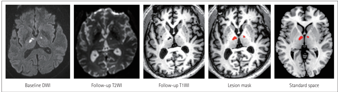
Supplementary Fig. 1. Representative case of lesion mask. For image preprocessing, we visually delineated the acute stroke lesions in DWIs obtained at the time of admission and superimposed the lesion mask on the volumetric T1WIs acquired 3 months after stroke using MRICron software. These lesion masks were used for the subsequent image preprocessing for volume reconstruction. DWI: diffusion-weighted image, T1WI: T1-weighted image, T2WI: T2-weighted image.
