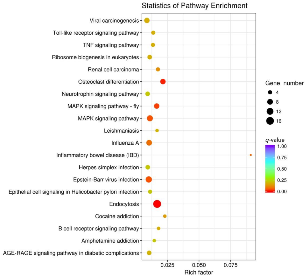
Figure S1. Results of KEGG enrichment.
