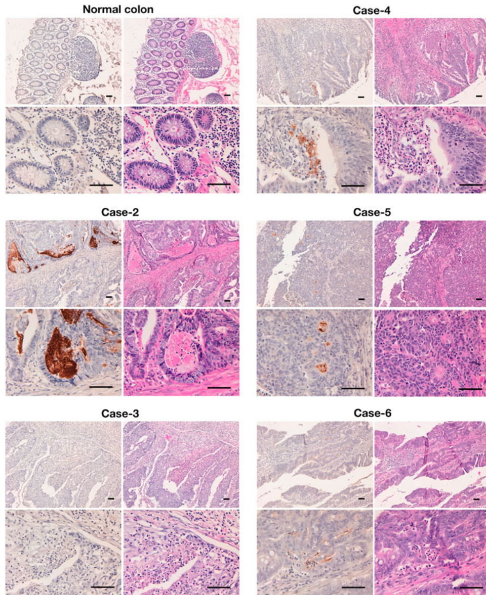
SUPPLEMENTARY FIG. S2. Immunohistochemical analysis of colon cancer by C Mab-43. Sections of normal colon and colon cancer (Case Nos. 2–6) were incubated with 1 μg/mL of C Mab-43, followed by the Envision+ kit. Color was developed using DAB and counterstained with hematoxylin. Serial sections were also stained using hematoxylin and eosin. Scale bar: 100 μm.
