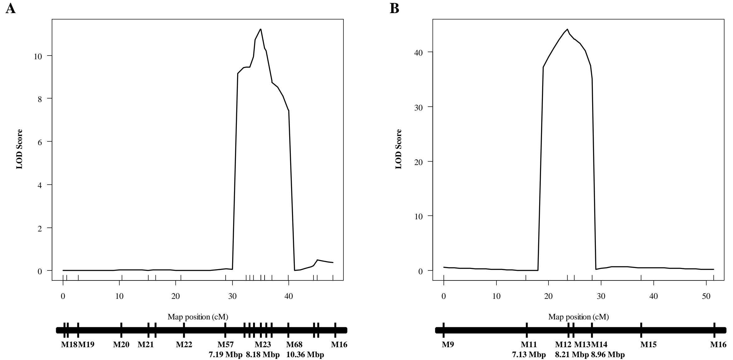
Supplemental Fig. 1. LOD profile obtained from composite interval mapping of M_Gly with AF-F 4 (A) and KF-F 2 (B) population on Gm11. Representative marker names and physical positions of these shown in supplemental table1 are displayed below of each graph.
