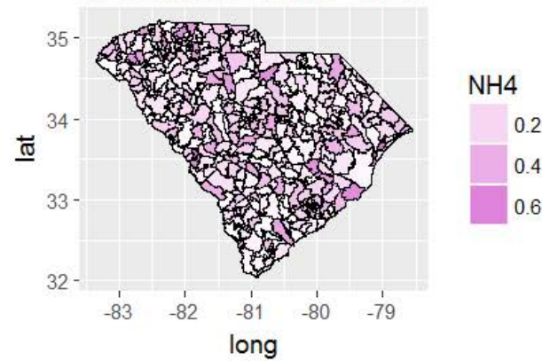
W Estimate Errors - NH4
