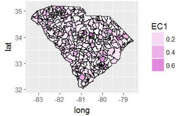
W Estimate Errors - EC1
