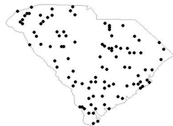
W Estimate Errors - EC1
