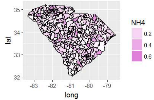
W Estimate Errors - NH4
