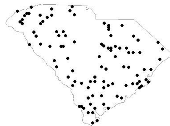
W Estimate Errors - EC1
