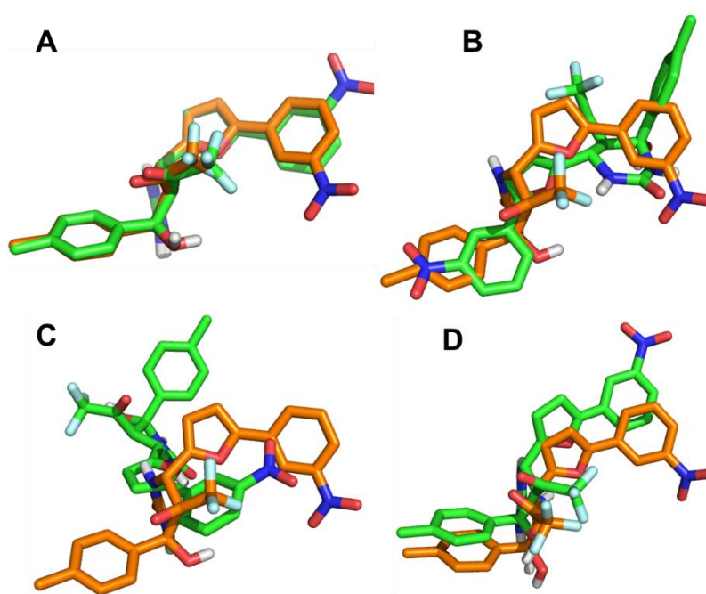
S3 Fig. Comparison between top docking poses and the representative conformations of the two clusters sampled by MD simulations. The Top 1 pose (docking score = -7.22 kcal/mol) is always shown as brownish sticks and three other poses are shown in greenish sticks: Docking Pose 2 (docking score = -6.66 kcal/mol) in Panel A, Docking Pose 3 (docking score = -6.55 kcal/mol) in Panel B and Docking Pose 4 (docking score = -6.48 kcal/mol) in Panel C. The representative conformations of Clusters 1 and 2 are shown as greenish and brownish sticks (Panel D).
