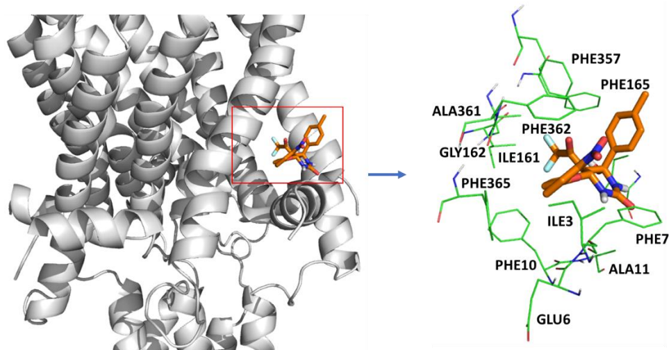
S5. Fig. Binding pocket (left) and the key residues interacting with K05 (right) for Docking Pose 4.
