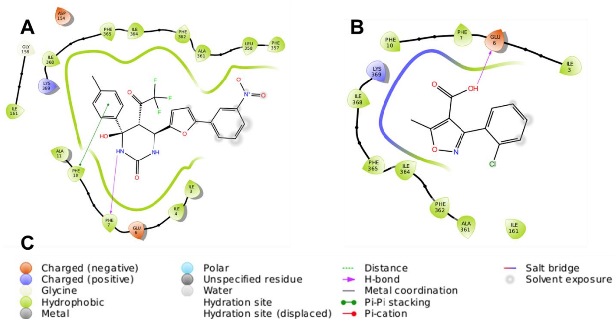
S6 Fig. 2D-Diagram of detailed interactions between K05 and Eco-MscL (Panel A), 011A and Eco-MscL (Panel B) reviewed by the best docking poses. The key of interaction types and sites is shown in Panel C.
