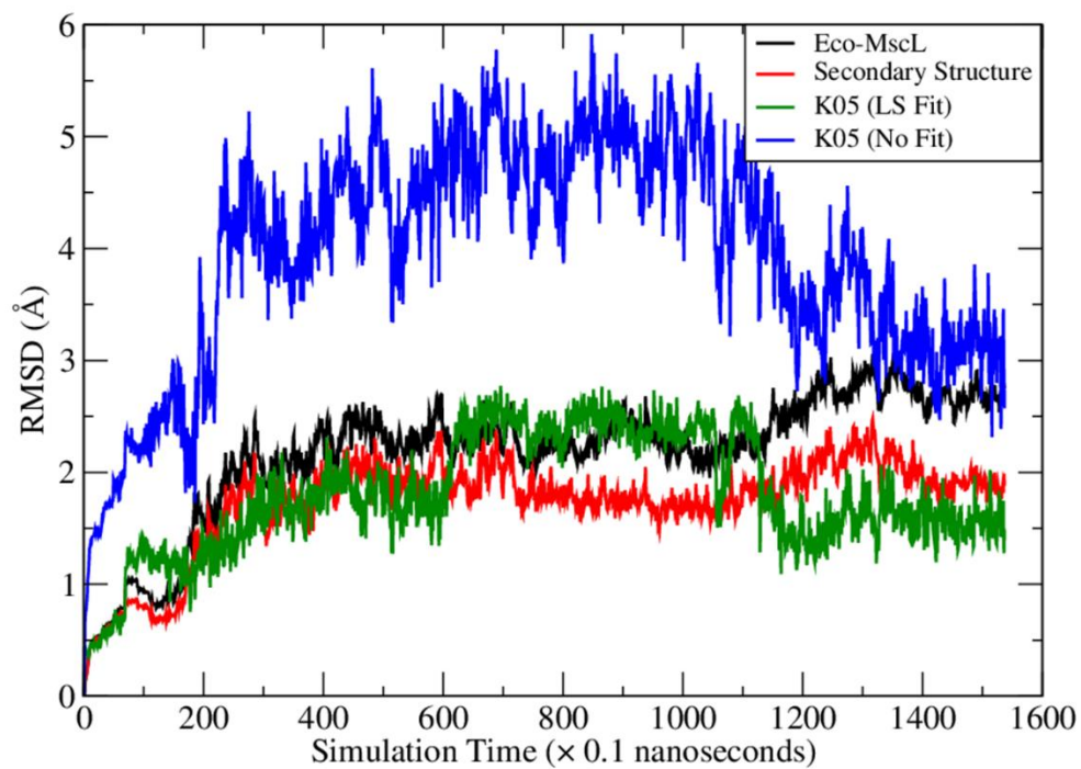
S8 Fig. The RMSD (Root-mean-square deviation) ~ Simulation Time plot for Docking Pose 1. According to the RMSDs of nonfit ligand (the blue curve), two conformation clusters can be observed. The first cluster is from 20 to 115 ns and second from 115 to 155 ns.
