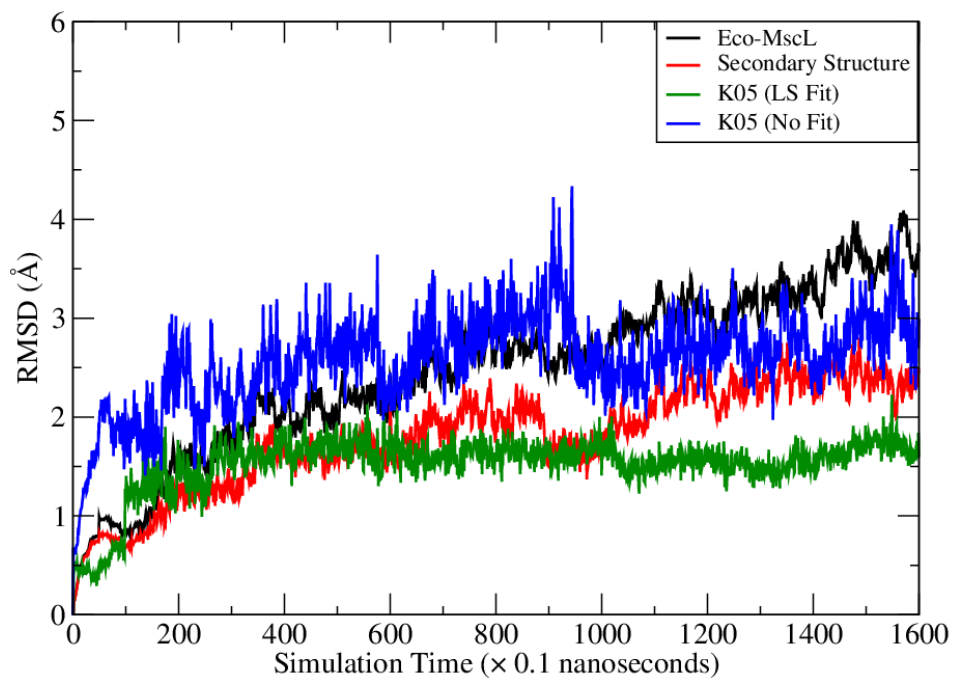
S10 Fig. The RMSD (Root-mean-square deviation) ~ Simulation Time plot for Docking Pose 3.
