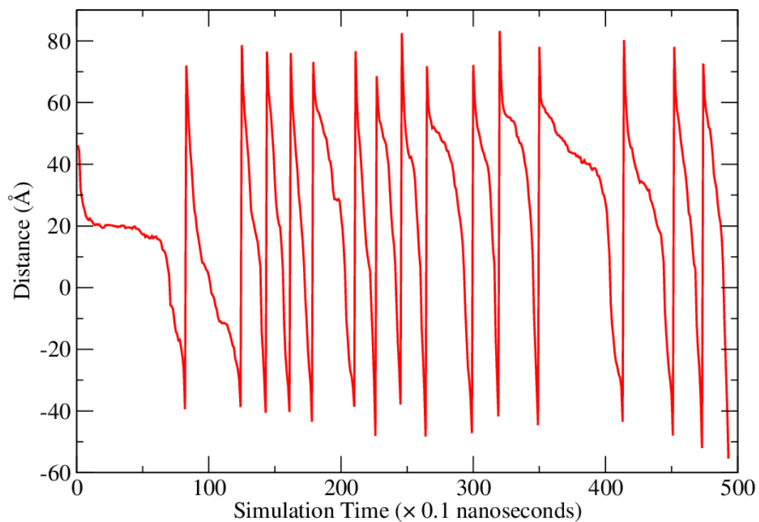
S12 Fig. Passing-through experiment induced by an external electric field of 0.2 Volt/Å applied to DHS. DHS passed through the MscL channel 15 times within 50 nanoseconds. The distance is between the center of the DHS and the center of five LYS106 residues.
