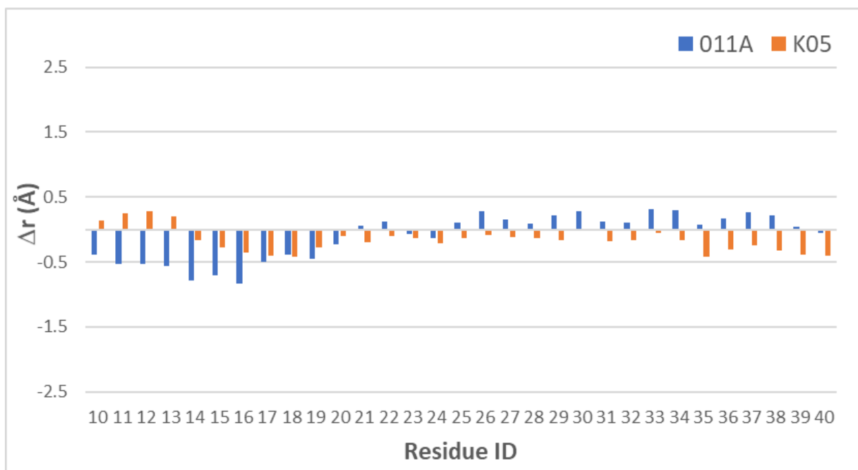
S13 Fig. The changes of channel radii upon ligand binding. \Delta r = r_{MscL/Lig} - r_{MscL} , where r_{MscL/Lig} is the channel radii for the MscL/011A or MscL/K05 complex and r_{MscL} is that for MscL protein only. The radii parameters were calculated for a set of MD snapshots from conventional MD simulations.
