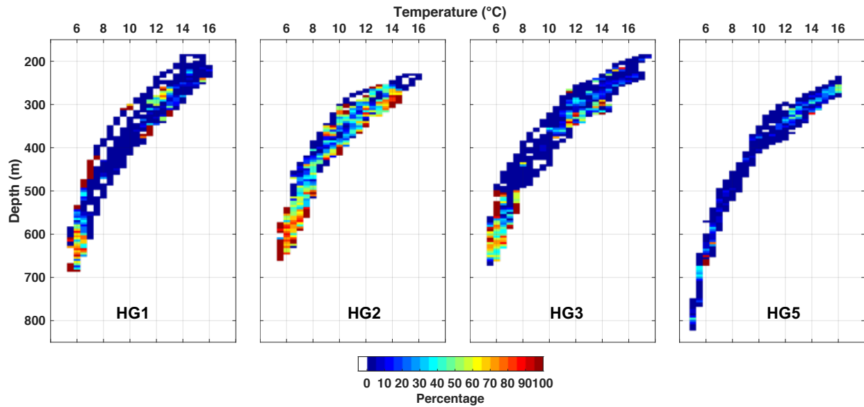
S7 Fig. Activity of sixgill sharks along a vertical profile of depth and ambient water temperature. Each grid cell ( 0.5 \text{ m} \times 0.5 \text{ }^\circ\text{C} ) is color-coded by the percentage of observations corresponding to the high-activity state (state 2) from the decoded state sequence derived from the best-fit hidden Markov model.
