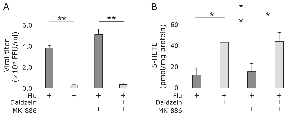
Supplemental Fig. 1. Effect of FLAP inhibitor, MK-886, on multiplication of influenza virus and production of 5-HETE. MDCK cells were inoculated with influenza A/PR/8/34 virus at a MOI of 0.001. (A) Effect of MK-886 on titer of influenza virus. Viral titers were determined at 24 h post-infection by focus-forming assays. (B) Effect of MK-886 on 5-HETE production. Data are presented as mean \pm SD ( n = 3 ). Data are representative of three independent experiments. * p < 0.005 , ** p < 0.001 .
