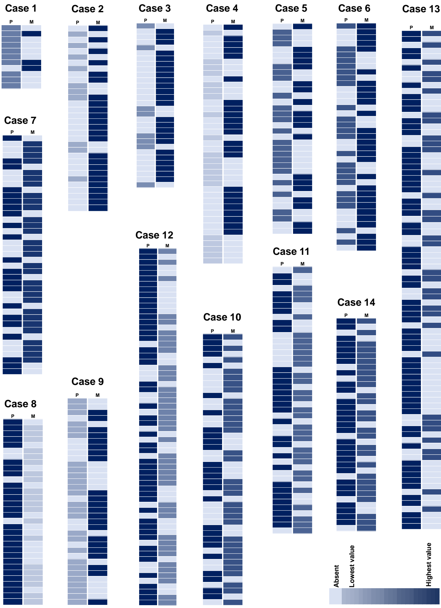
Supplementary Fig. 1: Somatic mutations in primary tumor and their metastatic lesions. Heatmaps show the variant allele fraction (VAF) of somatic mutations based on presence or absence as per the color key.
