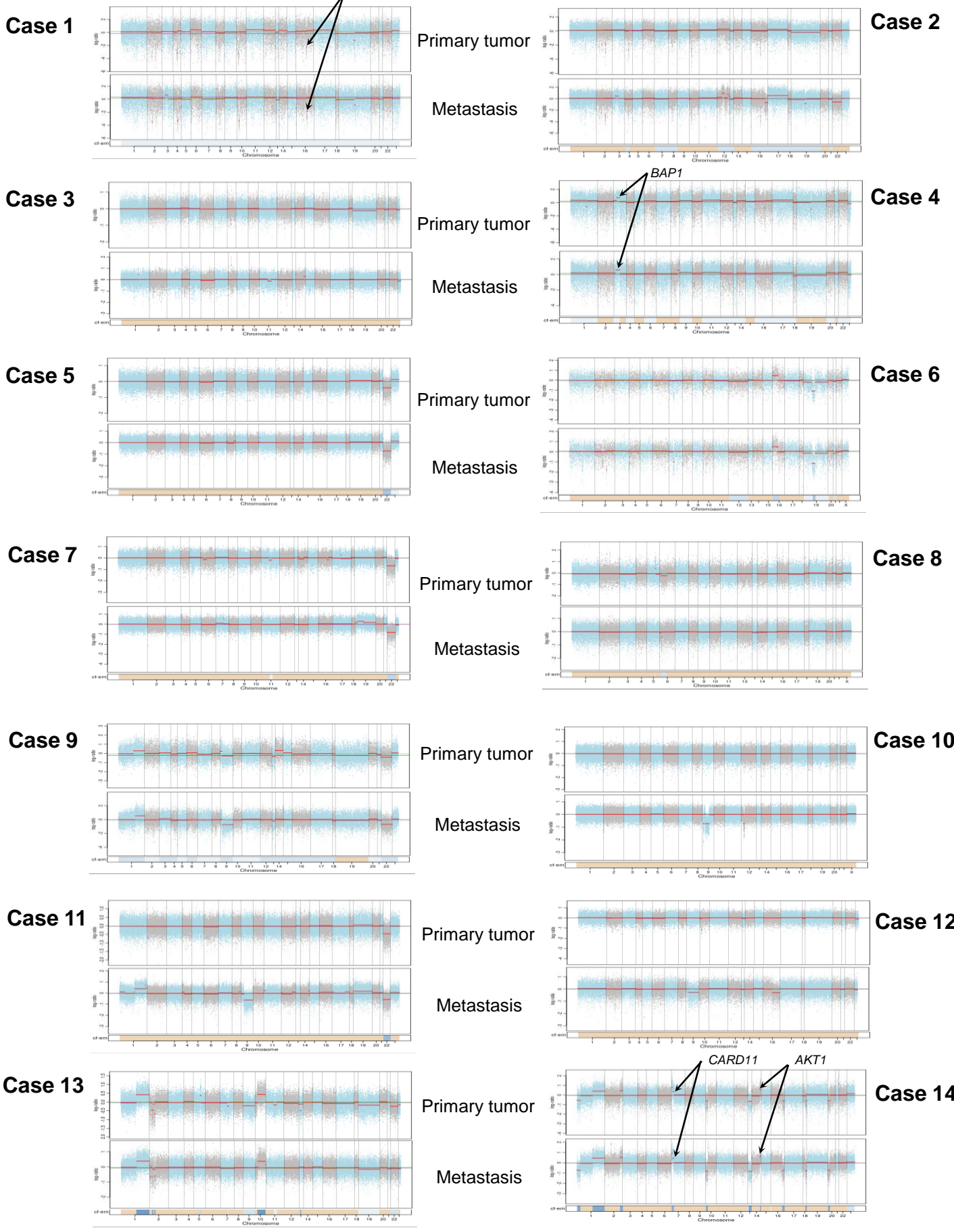
Supplementary Fig. 3: Genome plots of the primary tumor and their metastatic lesion. Segmented Log 2 ratios on y-axis were plotted according to their genomic positions on x-axis. Alternating blue and grey color demarcate the chromosomes. Black arrows indicates the shared focal amplifications and homozygous deletions in both lesions.
