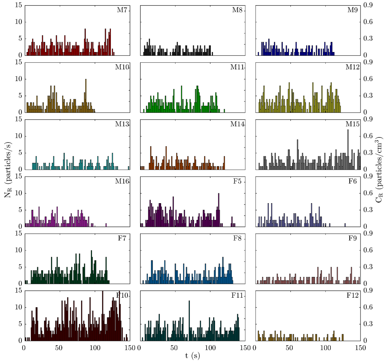
S4 Fig. Particle emission rate/concentration for reading Rainbow passage. Bar plots of particle emission rate/concentration versus time for reading Rainbow passage for 18 participants (10 males denoted as M7 to M16, and 8 females denoted as F5 to F12).
