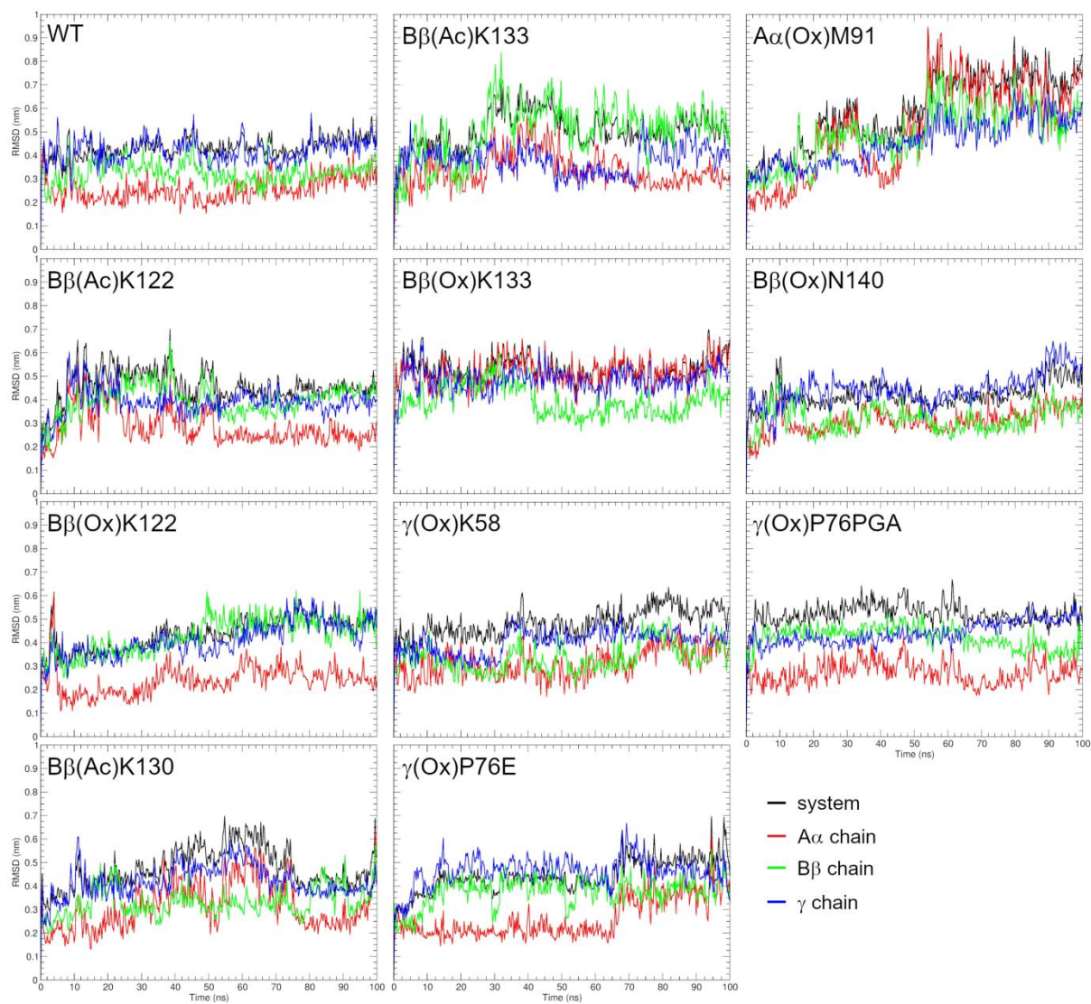
Fig S3. Development of RMSD of C _{\alpha} carbons in time for coiled-coil connector systems.
