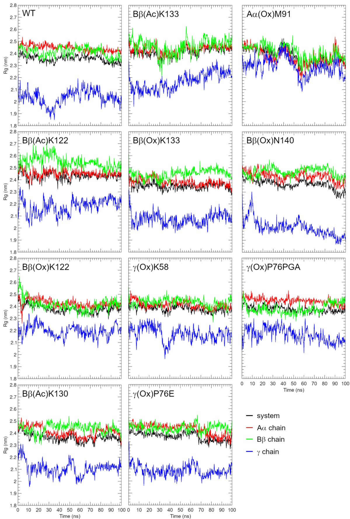
Fig S4. Development of radius of gyration of C_\alpha carbons in time for coiled-coil connector systems.
