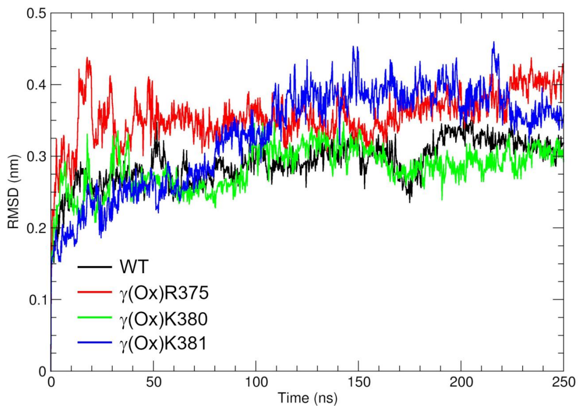
Fig S8. Development of RMSD of C_{\alpha} carbons in time for \gamma -nodule systems.
