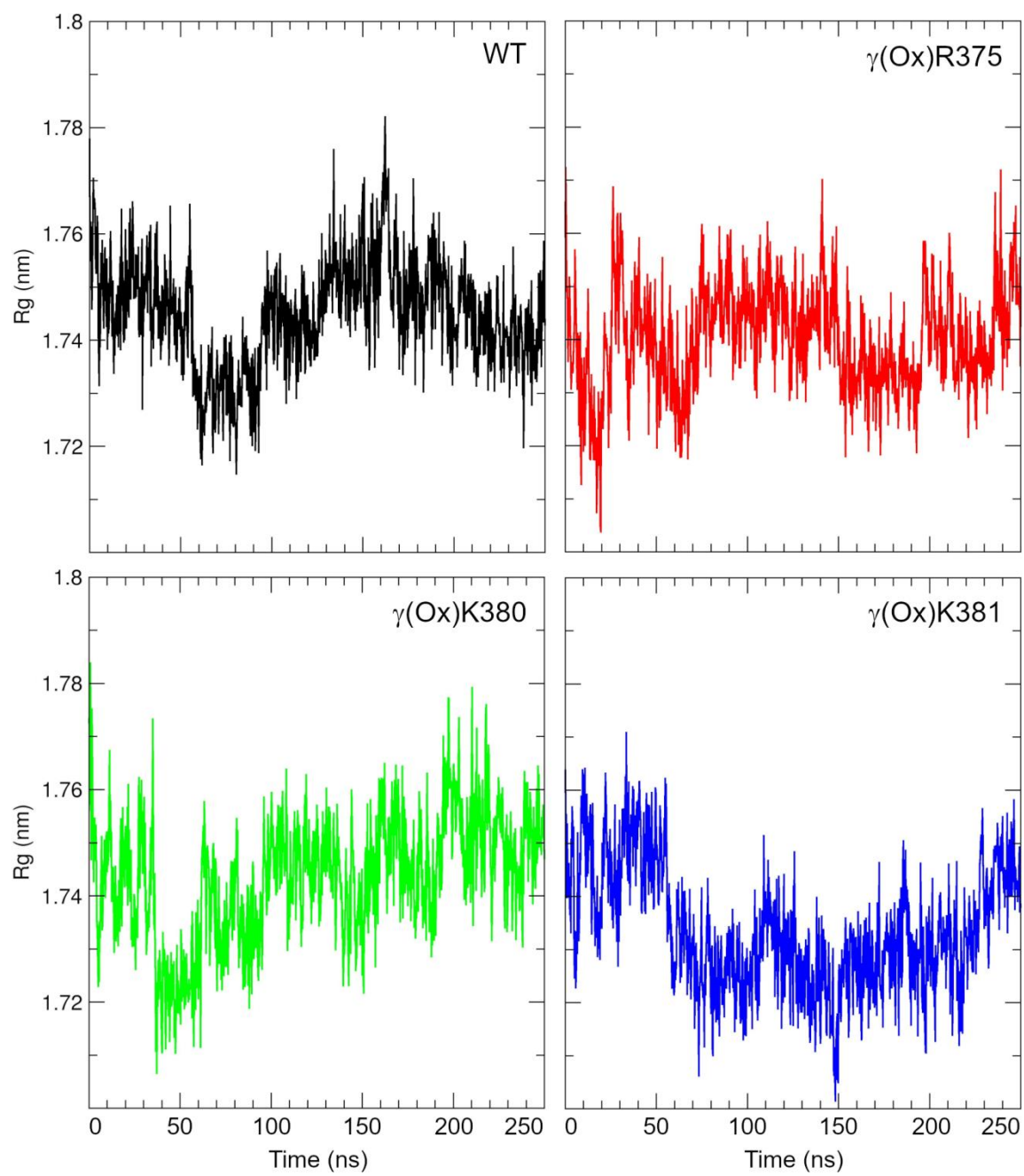
Fig S9. Development of radius of gyration of C_\alpha carbons in time for \gamma -nodule systems.
