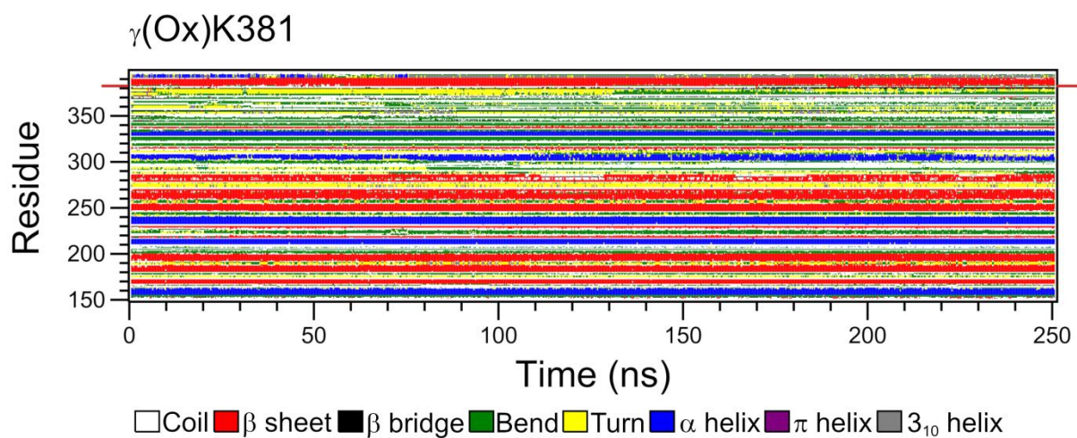
Fig S10. (all above) Development of secondary structure (DSSP) for systems examining \gamma -nodule of fibrinogen. Modified amino acid is highlighted by red bars at sides of plot.
