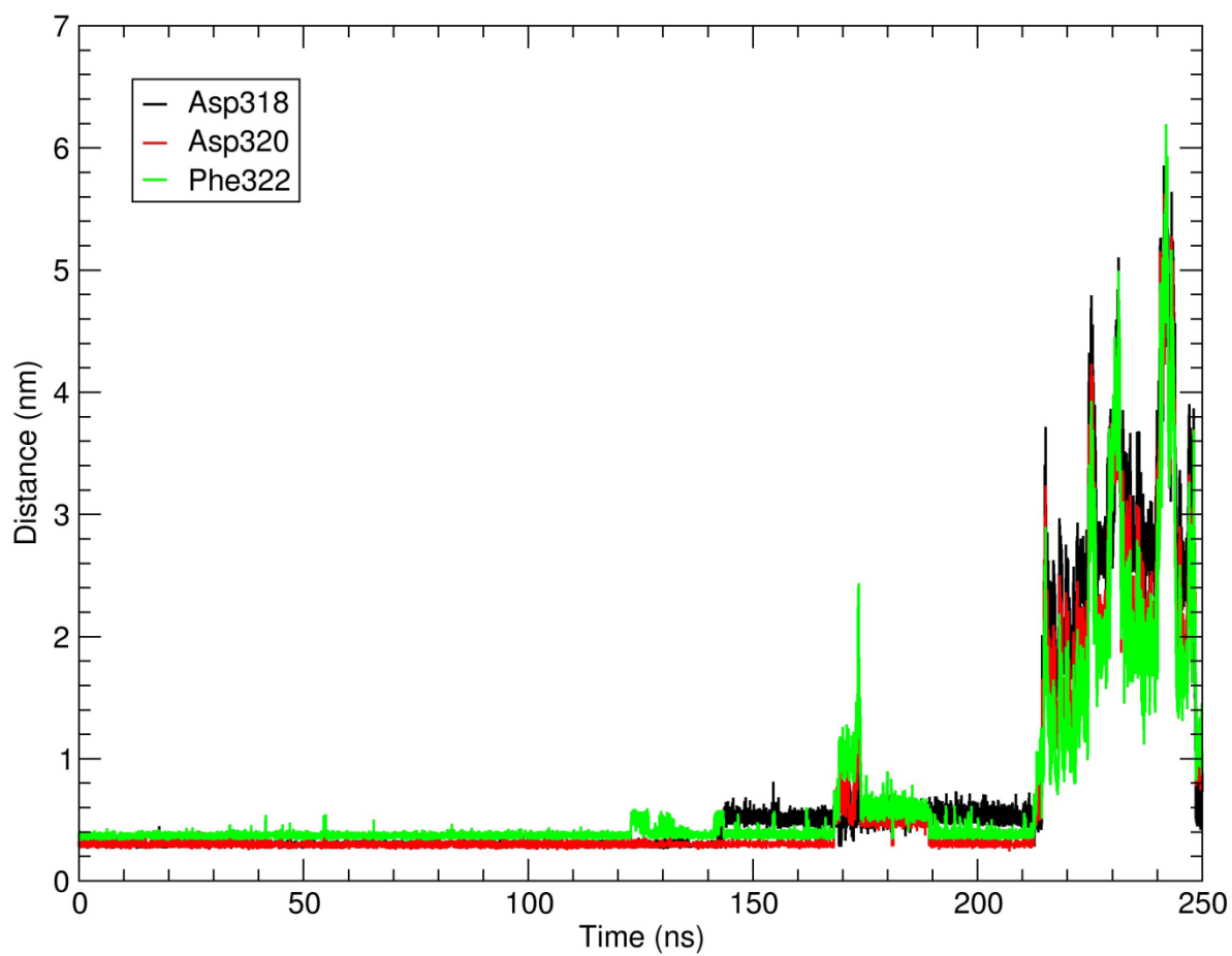
Fig S11. Unbinding of the \text{Ca}^{2+} ion. Distance of \text{Ca}^{2+} ion from \text{C}_\alpha carbons of \gamma\text{D318} (black), resp. \gamma\text{D320} (red) and from C carbon of \gamma\text{F322} (green) in dependence of time.
