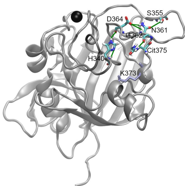
Fig S12. Hydrogen bond network formed as a result of oxidation of \gamma R375. Green lines show hydrogen bonds formed in the C-terminal part of the system with oxidized \gamma R375. In the WT simulation \gamma R375 forms hydrogen bond only with \gamma K373 (shown in violet). Carbon is shown in cyan, hydrogen in white, oxygen in red, nitrogen in blue and \text{Ca}^{2+} ion in black.
