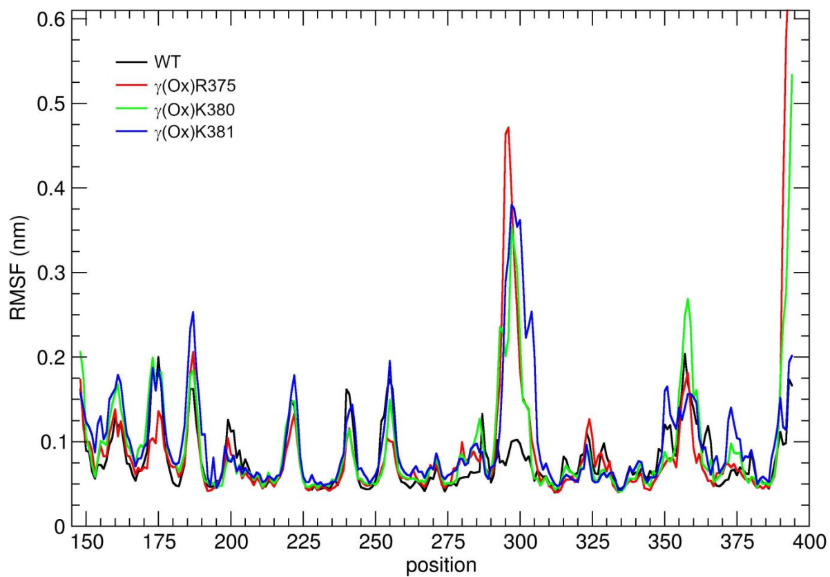
Fig S13. RMSF of C_{\alpha} carbons computed over the last 25 ns of simulations of the \gamma -nodule systems.
